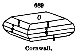
Cornwall.
